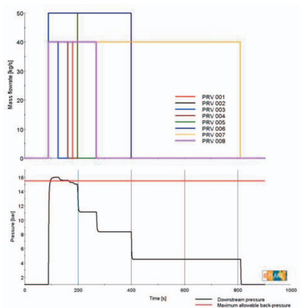
Figure 3. Option 1 backpressure profile for PRV 3 from dynamic simulation (lower) using square wave relief flows (upper).
